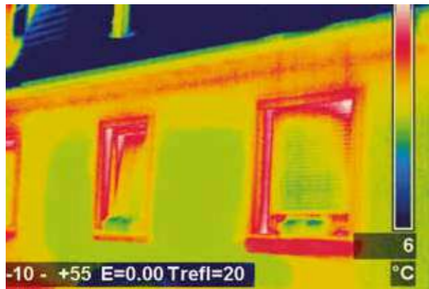
The warmest areas seen here in red show where heat is being lost from the building.
